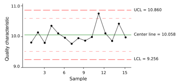
Figure 5 Control Chart
