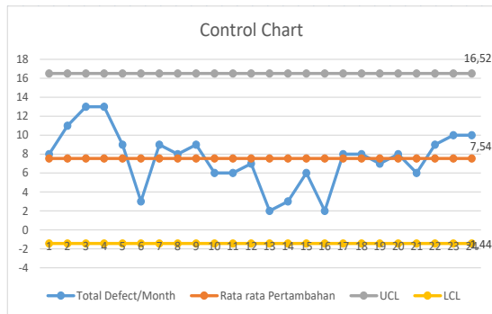
Figure 9 Control Chart
